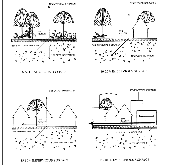
Figure 2. Effects of different levels of impervious surfaces on infiltration and runoff of rain water.
